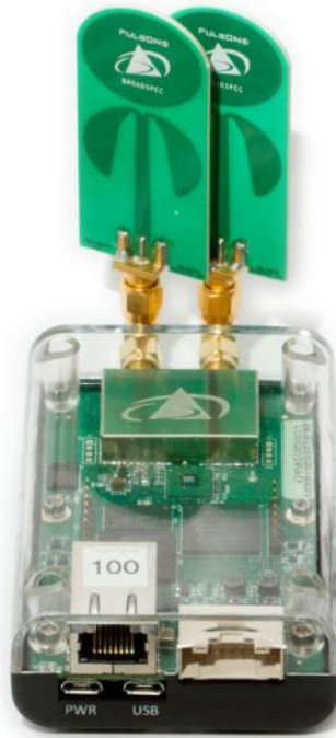
Fig. 1: P440 MRM with attached Broadspec Antennas
