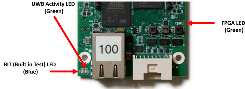
Fig. 5: Indicating LEDs
