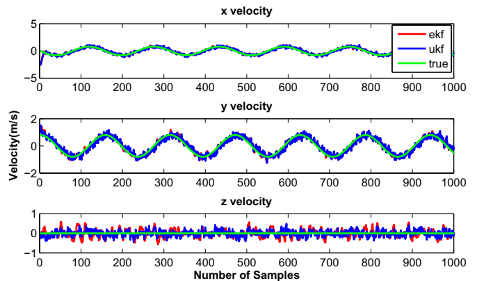
(b) EKF and UKF indoor velocity
