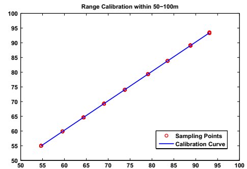
(c) Corridor calibration 50–100 m
