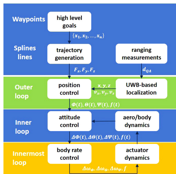
Fig. 13. Indoor autonomous flight workflow.
