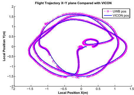
(a) Flight trajectory in x - y plane
