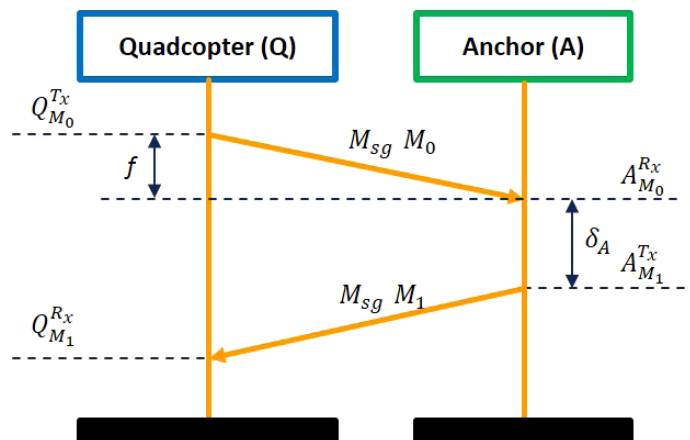
Fig. 1. TW-ToF range measurement.
