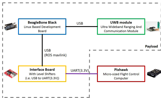
Fig. 7. Hardware architecture.
