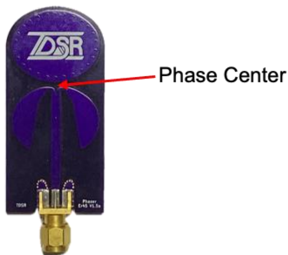
Fig. B-2: TDSR BroadSpec UWB antenna with radiating point indicated
