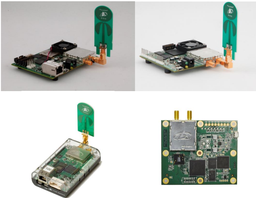
Fig. 1-A: Clockwise from upper left P400, P410, P412, and P440 (shown with attached BroadSpec Antenna)
